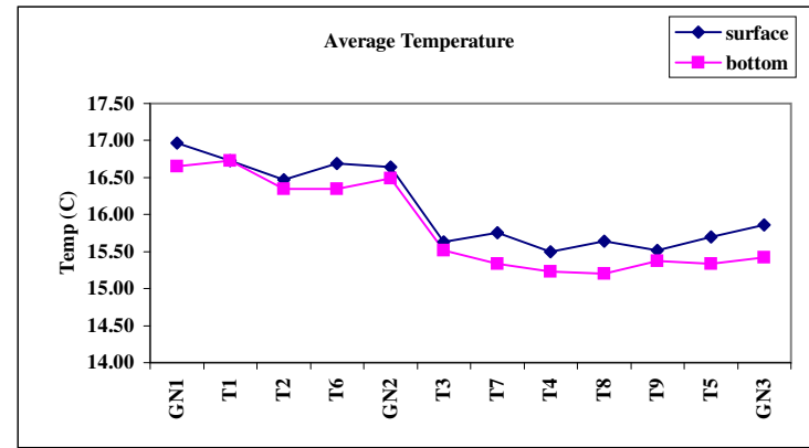
FIGURE 14 Water Quality Averages by Site Location NJMC/MERI Hackensack River Fishery Resource Inventory August 2001 to September 2003
